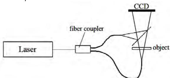
Fig. 1.1. Digital holographic microscope
