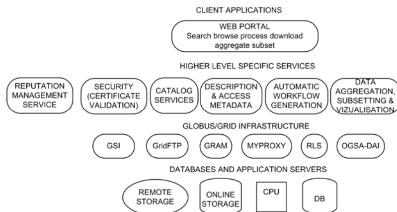
Fig. 3. System architecture
